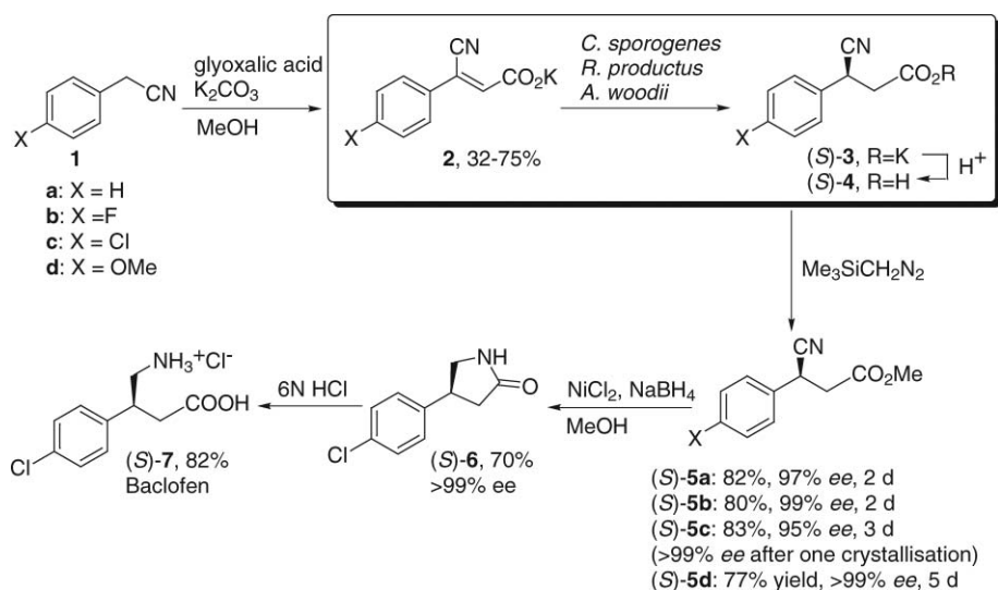
Scheme 1 Chemoenzymatic asymmetric synthesis of \beta -aryl- \gamma -amino acids.
